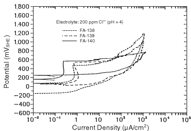
FIGURE 6. Effect of Mo content on the cyclic anodic polarization behavior of 4 at% Cr iron aluminides, FA-138, FA-139, and FA-140 in aerated 200 ppm \text{Cl}^- (pH = 4).
